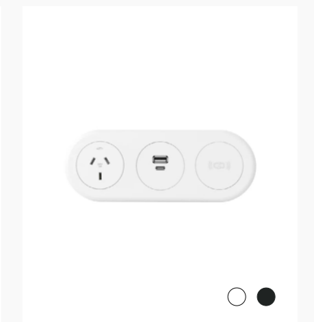
Echo Trio 1x GPO, USB A/C and Wireless Fast- Charge Module (1000mm Tag Lead)
