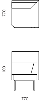
CAP-35 Corner mid-back seat – square
