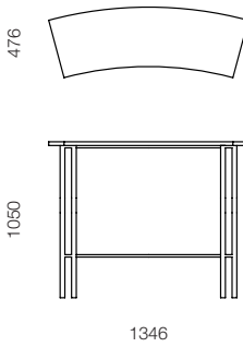
CAP-58 Curved seater bar table – 30 degree
