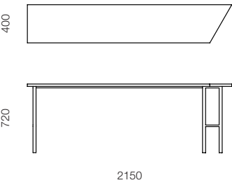
CAP-59L Angled two seater console table – left end
