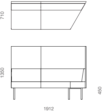
CAP-32L Angled high-back two seater – left end
