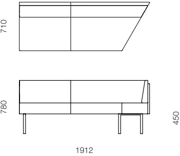
CAP-30L Angled two seater – left end
