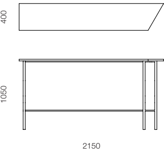
CAP-61L Angled two seater bar table – left end
