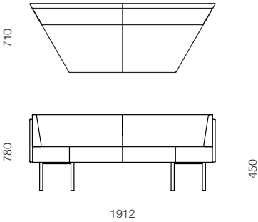
CAP-26 Angled two seater
