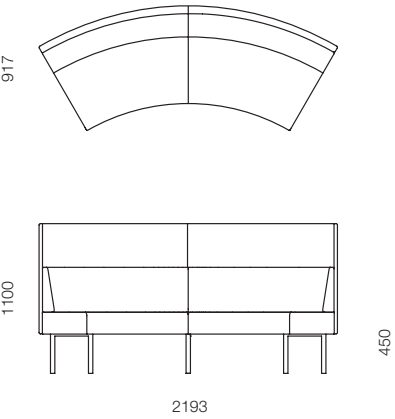
CAP-19 Curved mid-back two seater – 60 degree
