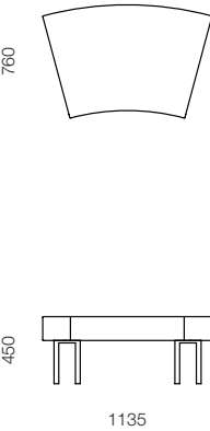
CAP-21 Curved single seater bench – 30 degree
