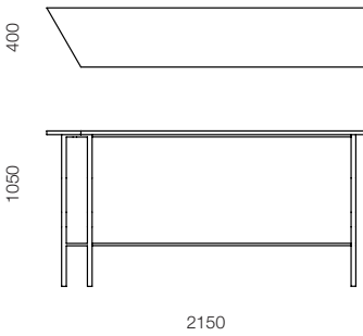
CAP-61R Angled two seater bar table – right end
