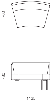
CAP-22 Curved single seater – 30 degree
