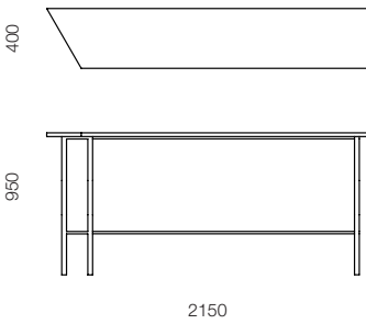
CAP-60R Angled two seater counter table – right end
