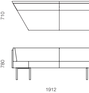
CAP-30R Angled two seater – right end
