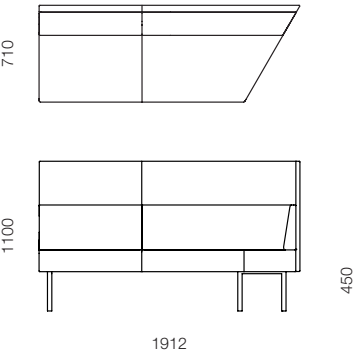
CAP-31L Angled mid-back two seater – left end
