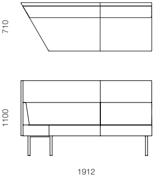
CAP-31R Angled mid-back two seater – right end
