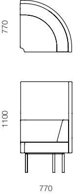
CAP-40 Corner high-back seat – round
