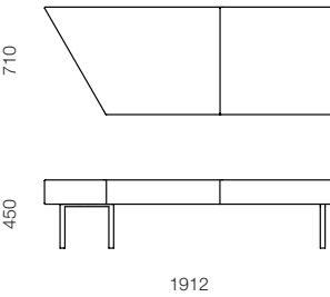
CAP-29R Angled two seater bench – right end
