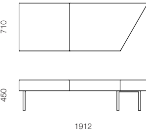
CAP-29L Angled two seater bench – left end
