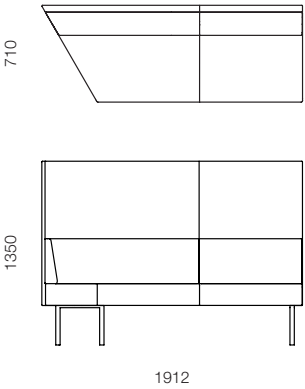
CAP-32R Angled high-back two seater – right end
