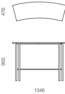
CAP-57 Curved seater counter table – 30 degree
