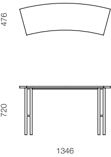
CAP-56 Curved seater console table – 30 degree
