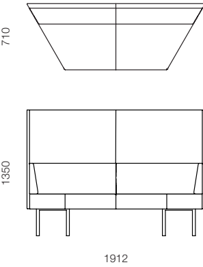
CAP-28 Angled high-back two seater
