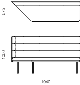
WAL-02R-F Freestanding banquette seat – right end
