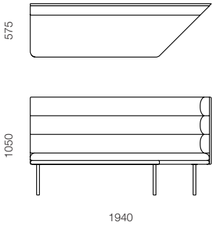
WAL-02L-F Freestanding banquette seat – left end
